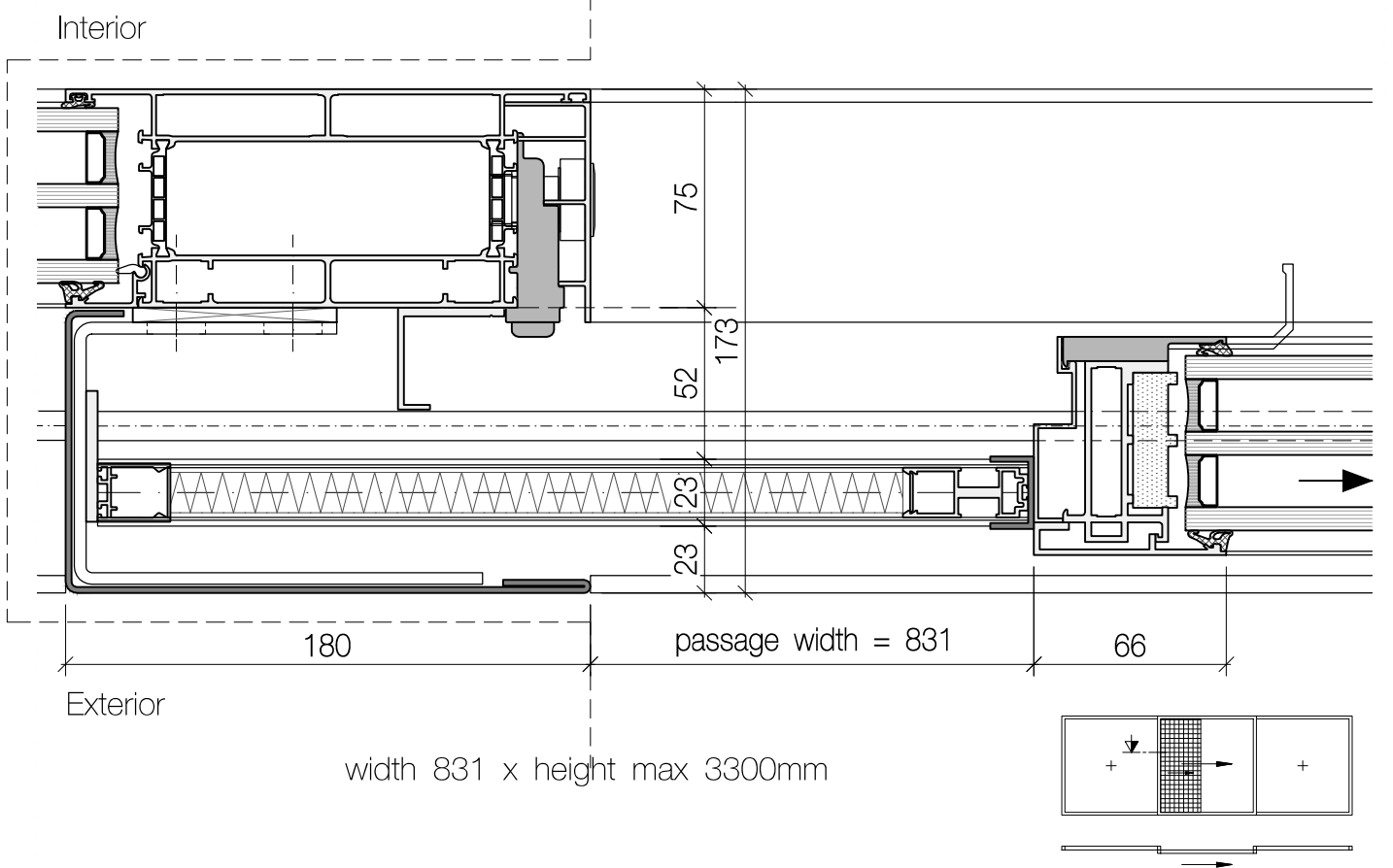
detail open sliding casement
