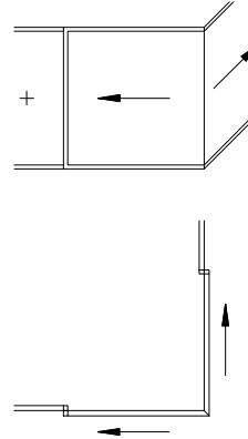
Exterior cornering with fully glazed pane
