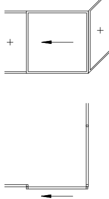
Exterior cornering with support post abutment
