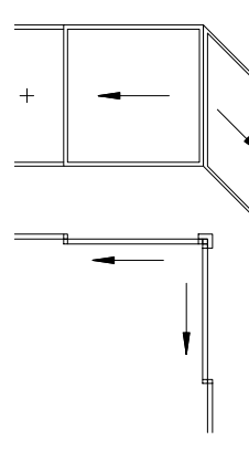
Interior cornering with support post abutment
