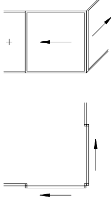
Exterior cornering with support post abutment
