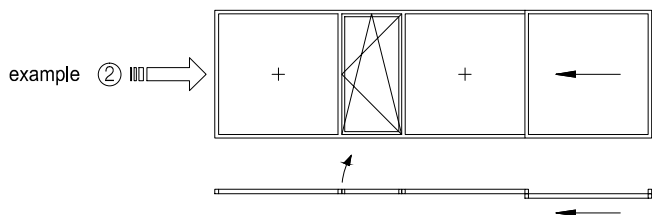
example ② 1 right casement sliding left over the right central fixed pane together with 1 left central swivel-opening casement and 1 left fixed pane
