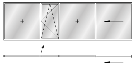
Sliding window schema A and tilt-and-turn window
