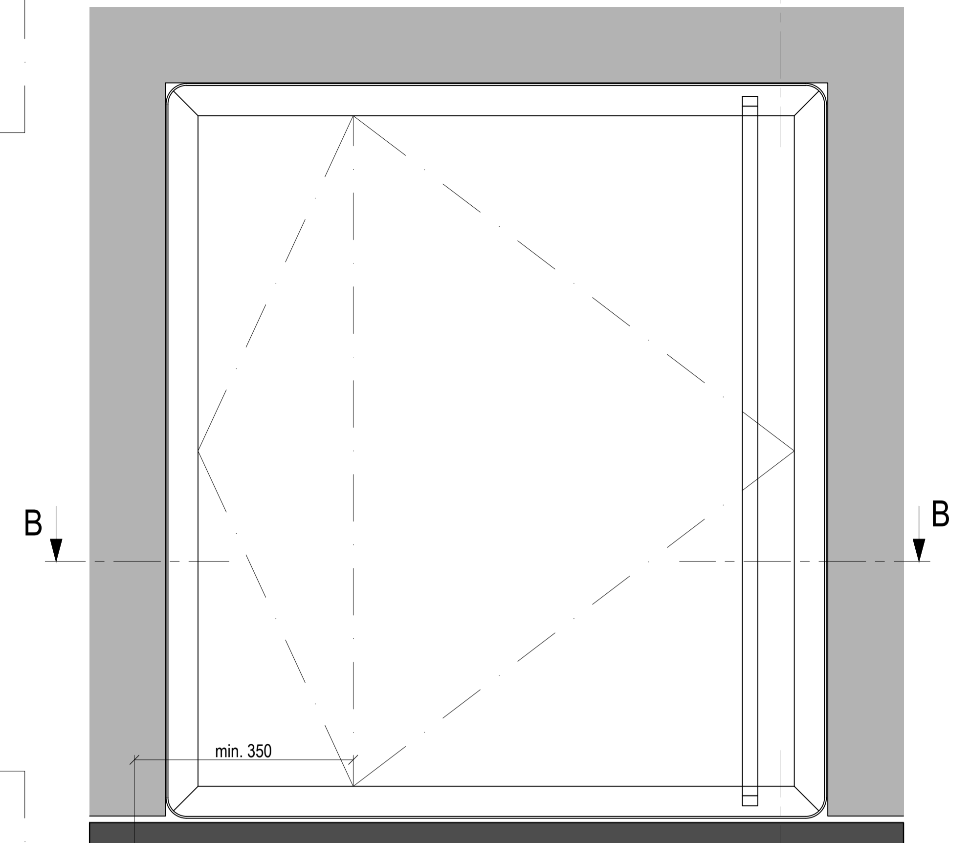
Pivot Door PD-75 Scale = 1 : 10
