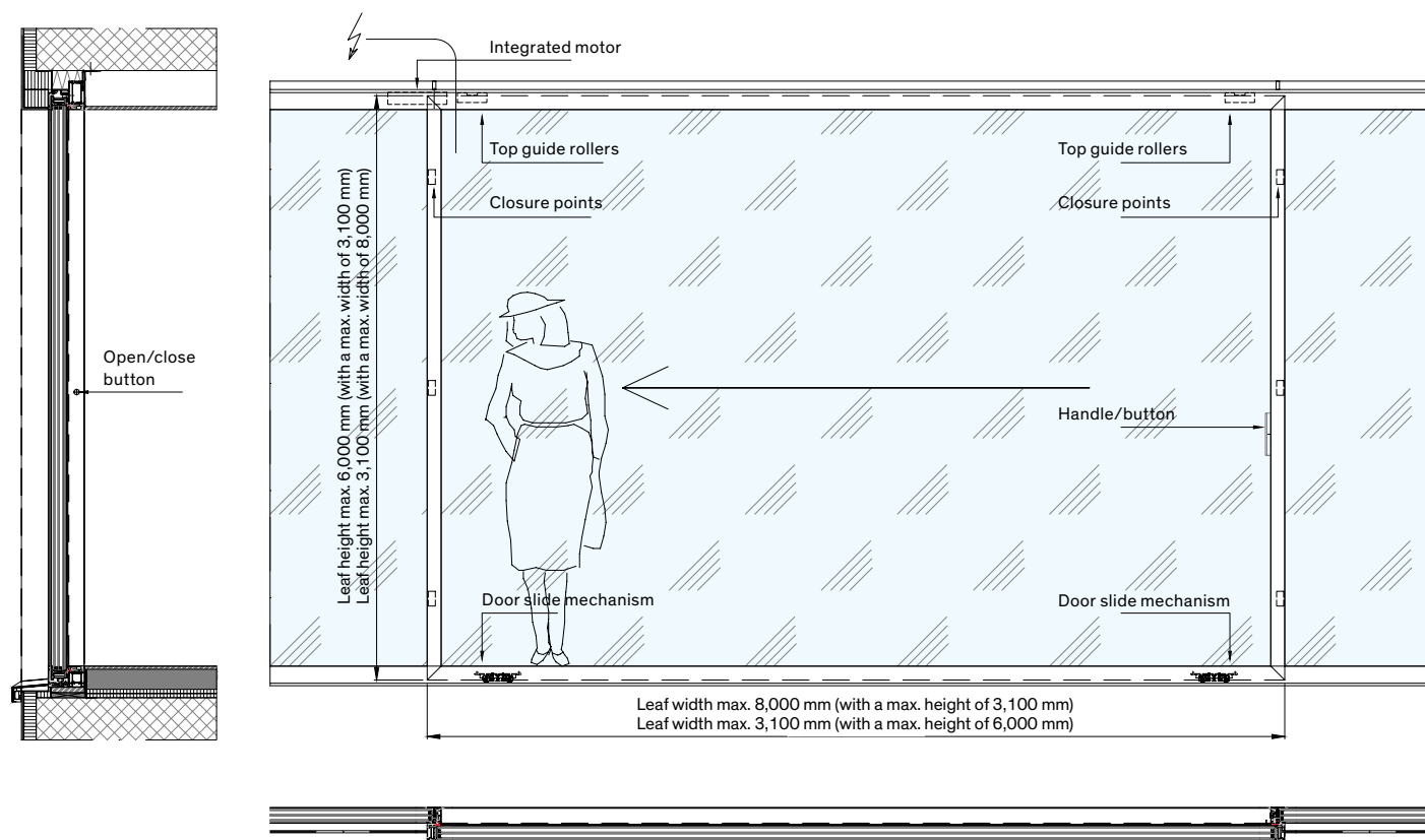
Vertical cross-section/view
